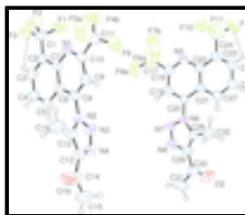
Fig. 1. The molecular structure of the title compound. Displacement ellipsoids are drawn at the 50% probability level. Hydrogen atoms are shown as spheres of arbitrary radius and showing intramolecular hydrogen bonds as dashed lines.
