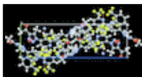
Fig. 2. Packing of the molecules showing hydrogen bonds as dashed lines.
